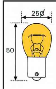
BA15s (special)
