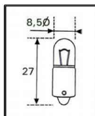
BA-9s
