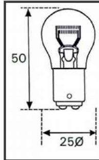
BAY15d (Off center)
